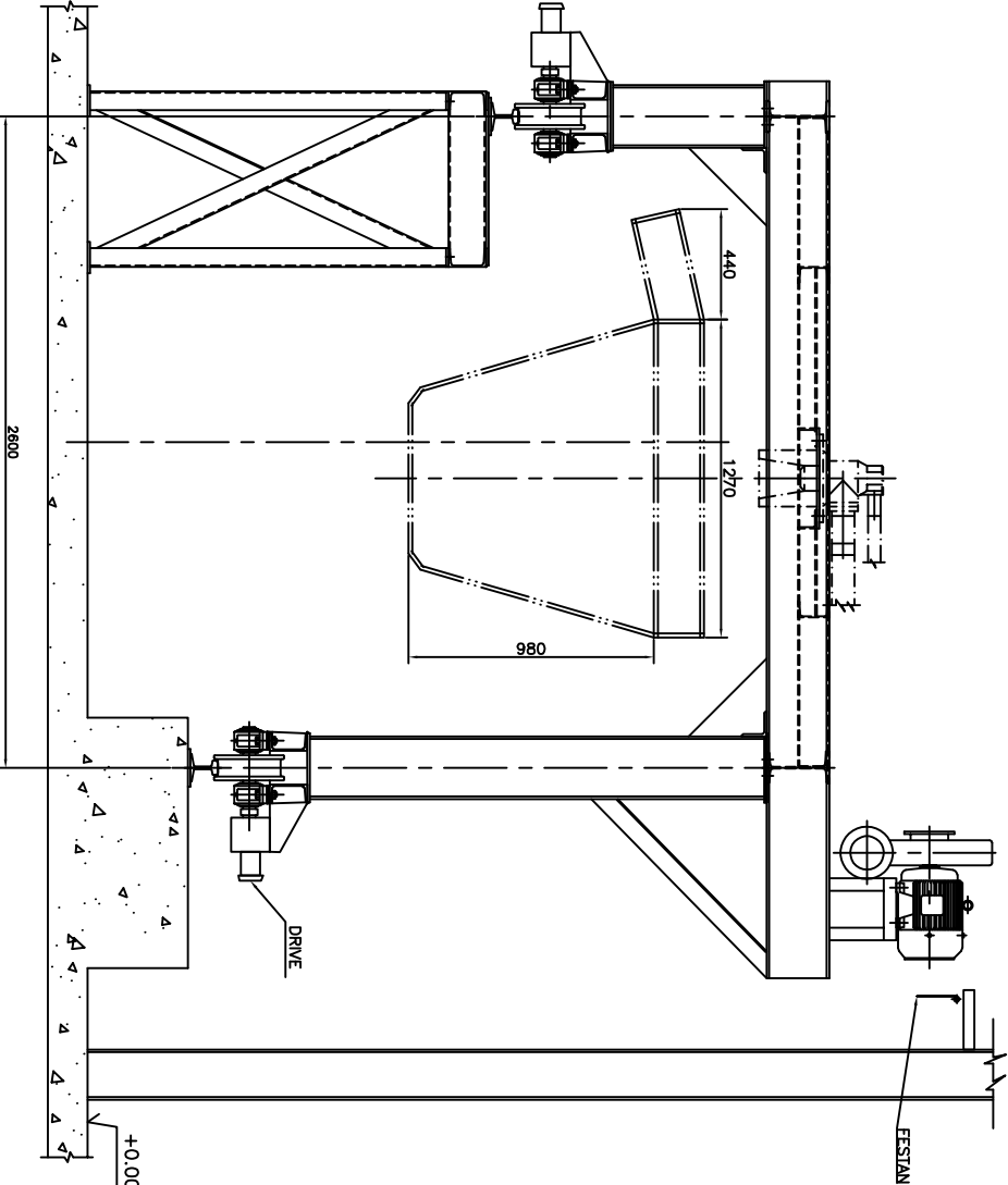
TUNDISH PREHEATER / DRYER
